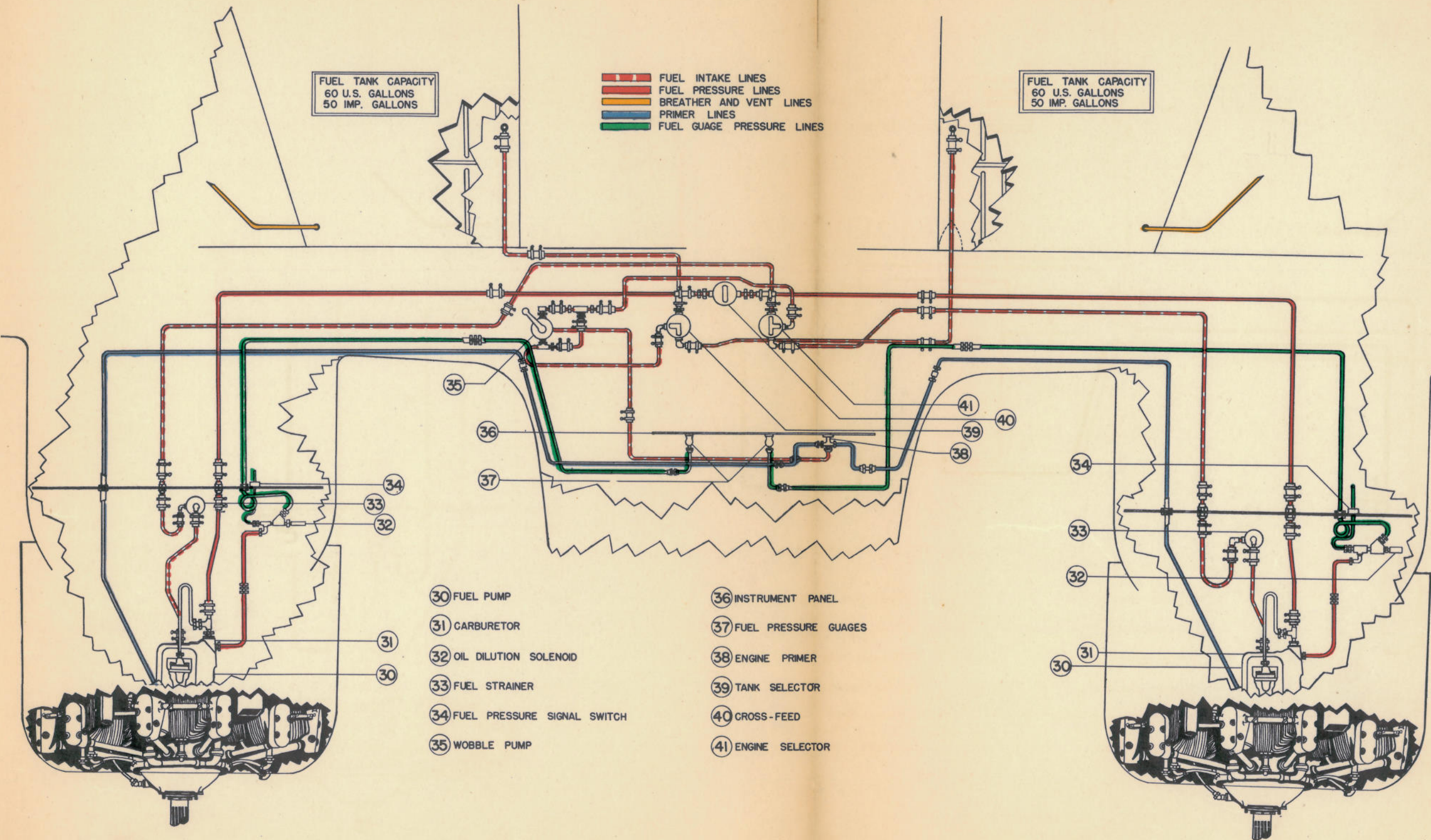
Figure 5 - Fuel System Diagram
